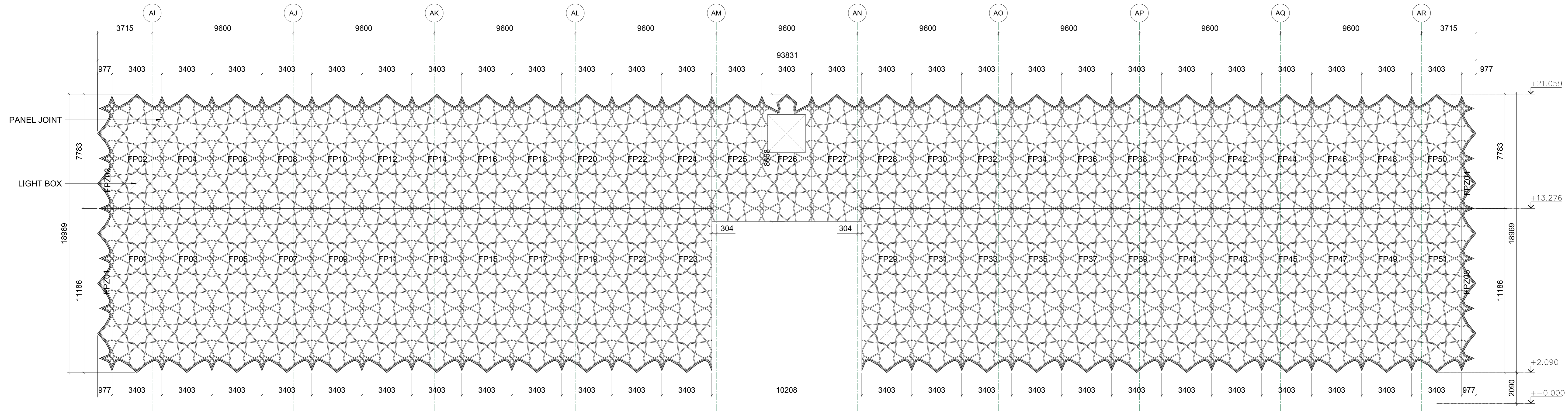
Front Wall Panel General Arrangement (with tiling pattern) Scale: 1/120
